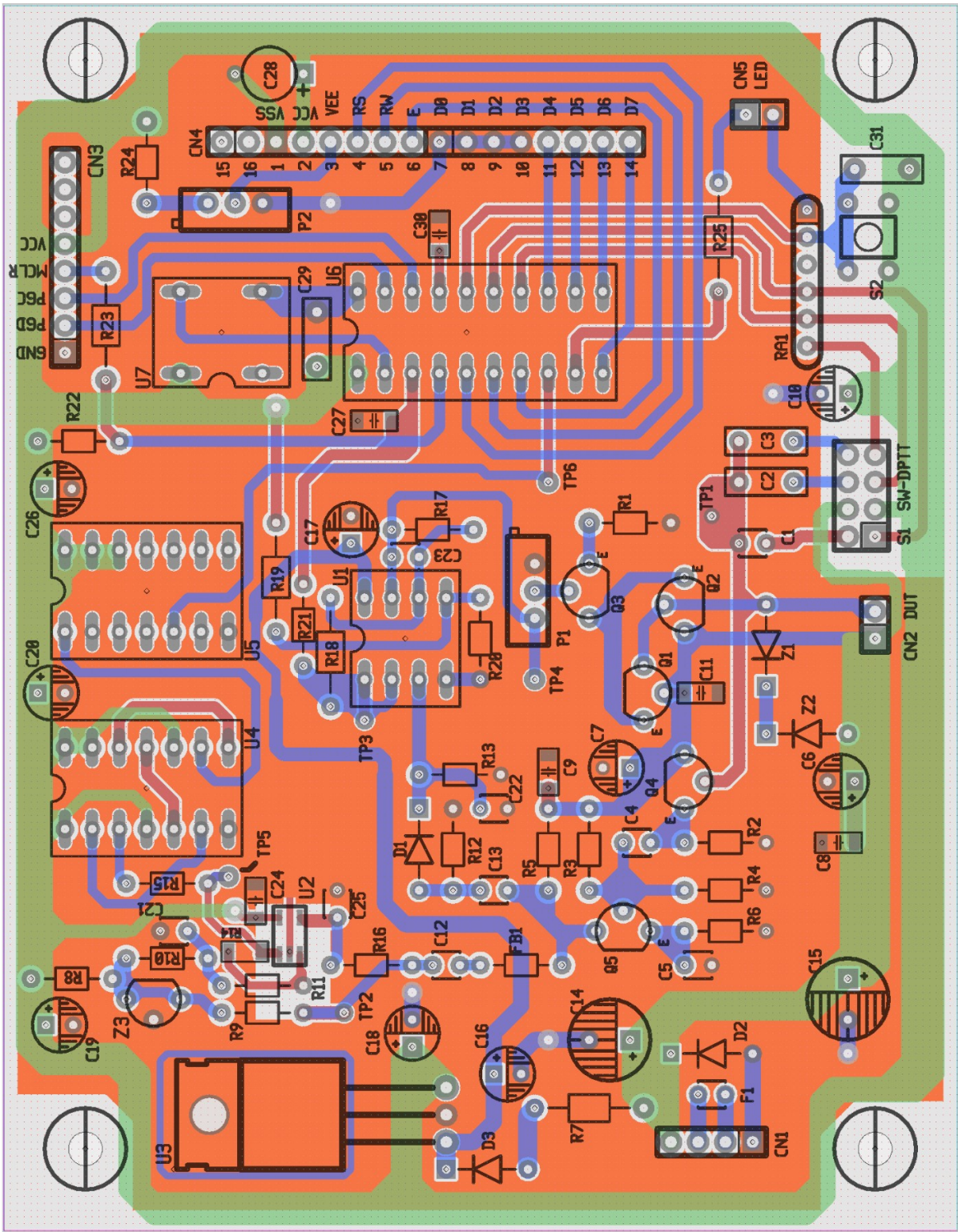
PCB Layout with Component Placement
